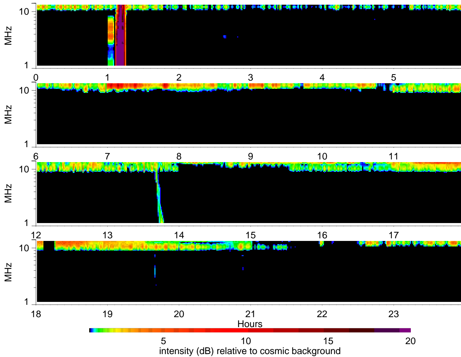
Wind Waves RAD2 receiver: 1995/6/11
