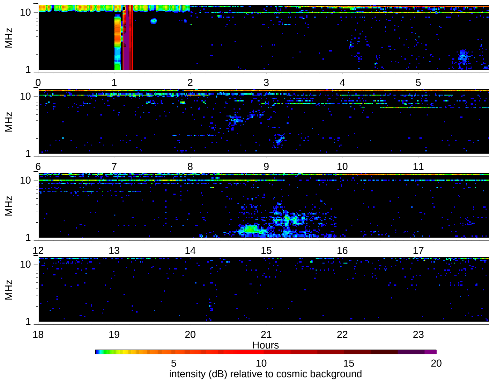
Wind Waves RAD2 receiver: 1995/6/13
