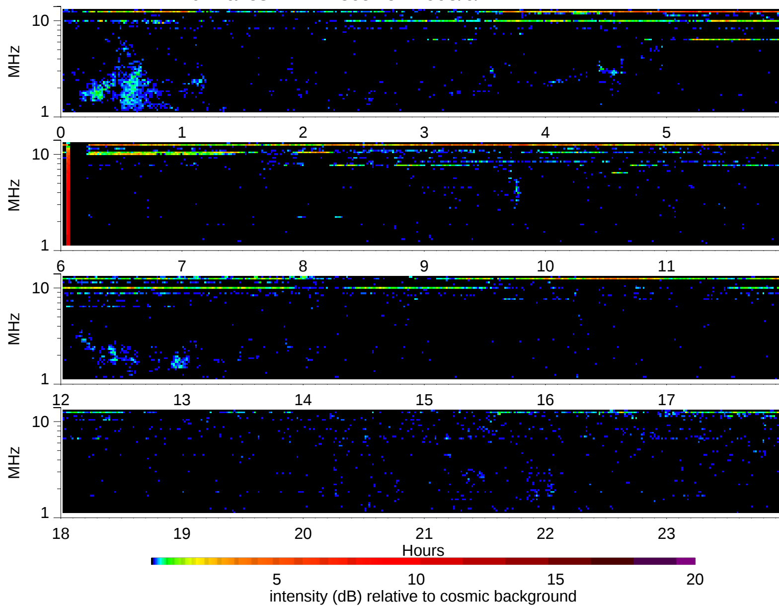
Wind Waves RAD2 receiver: 1995/6/14
