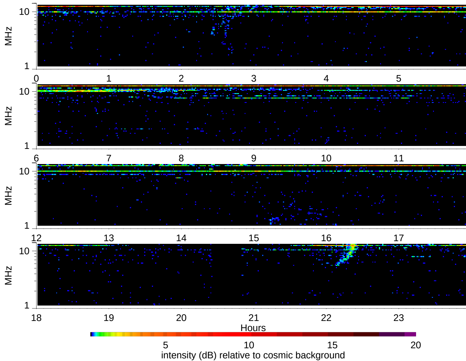
Wind Waves RAD2 receiver: 1995/6/15
