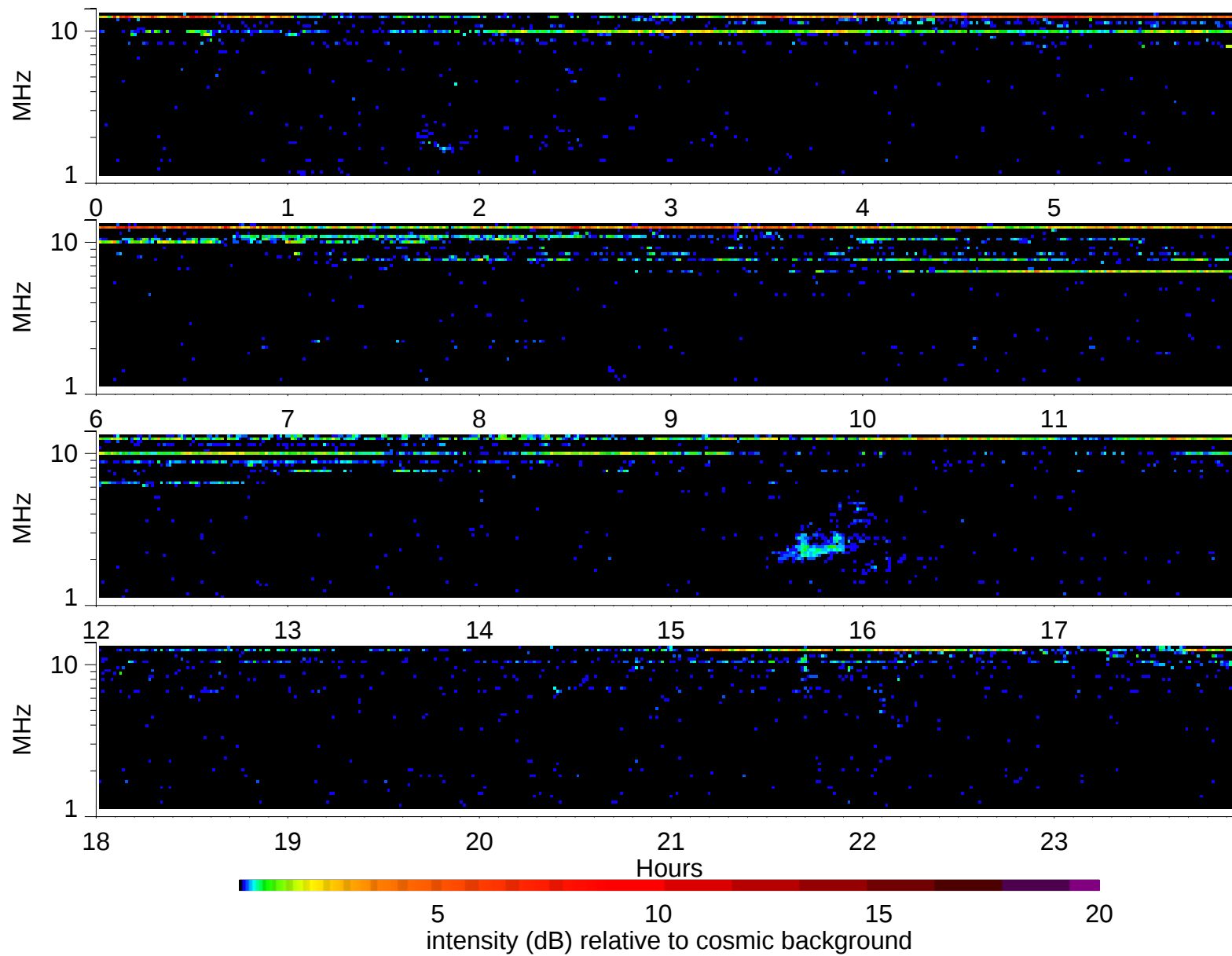
Wind Waves RAD2 receiver: 1995/6/16
