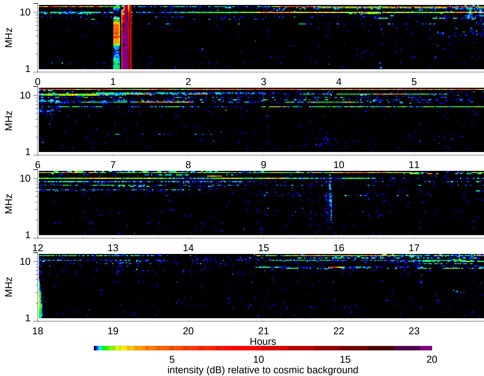
Wind Waves RAD2 receiver: 1995/6/21
