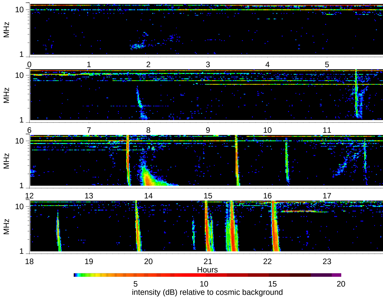
Wind Waves RAD2 receiver: 1995/6/24
