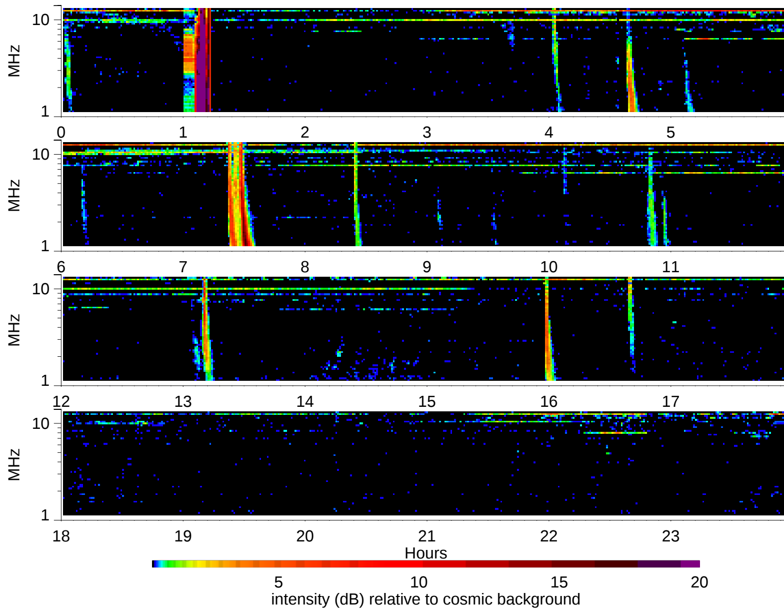
Wind Waves RAD2 receiver: 1995/6/25
