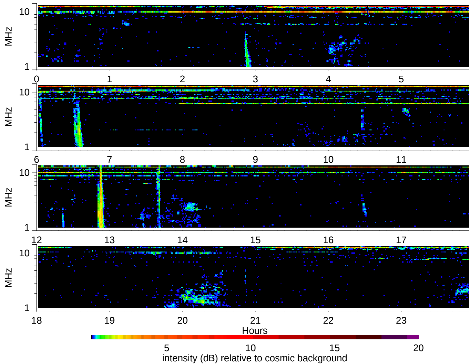
Wind Waves RAD2 receiver: 1995/6/26
