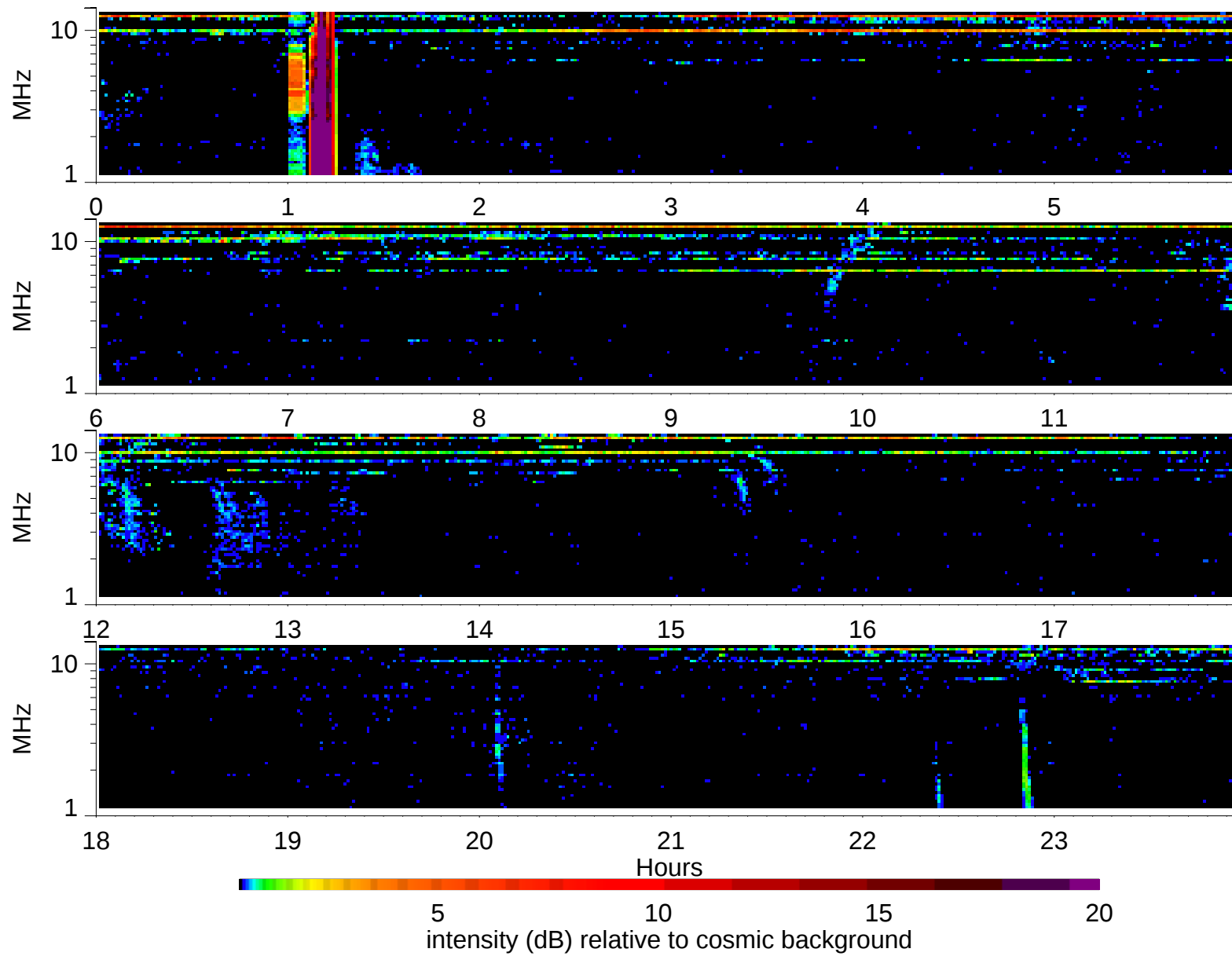
Wind Waves RAD2 receiver: 1995/6/27
