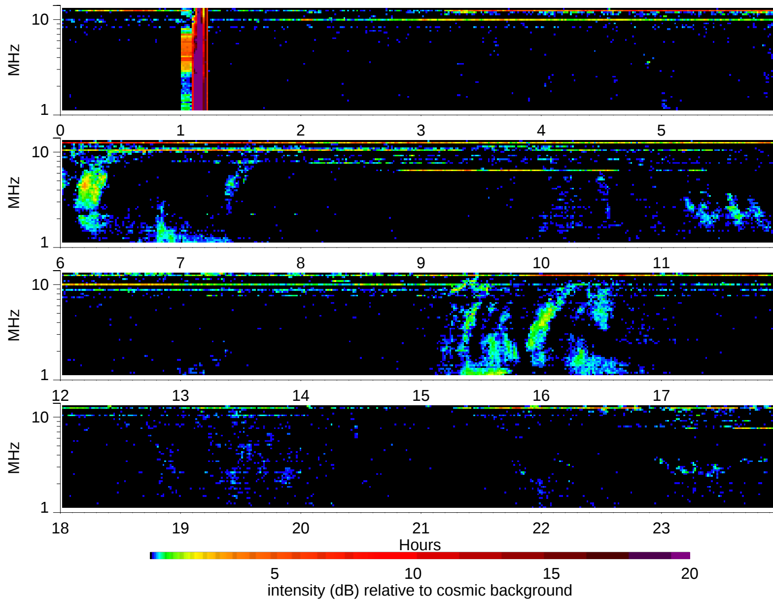
Wind Waves RAD2 receiver: 1995/7/3
