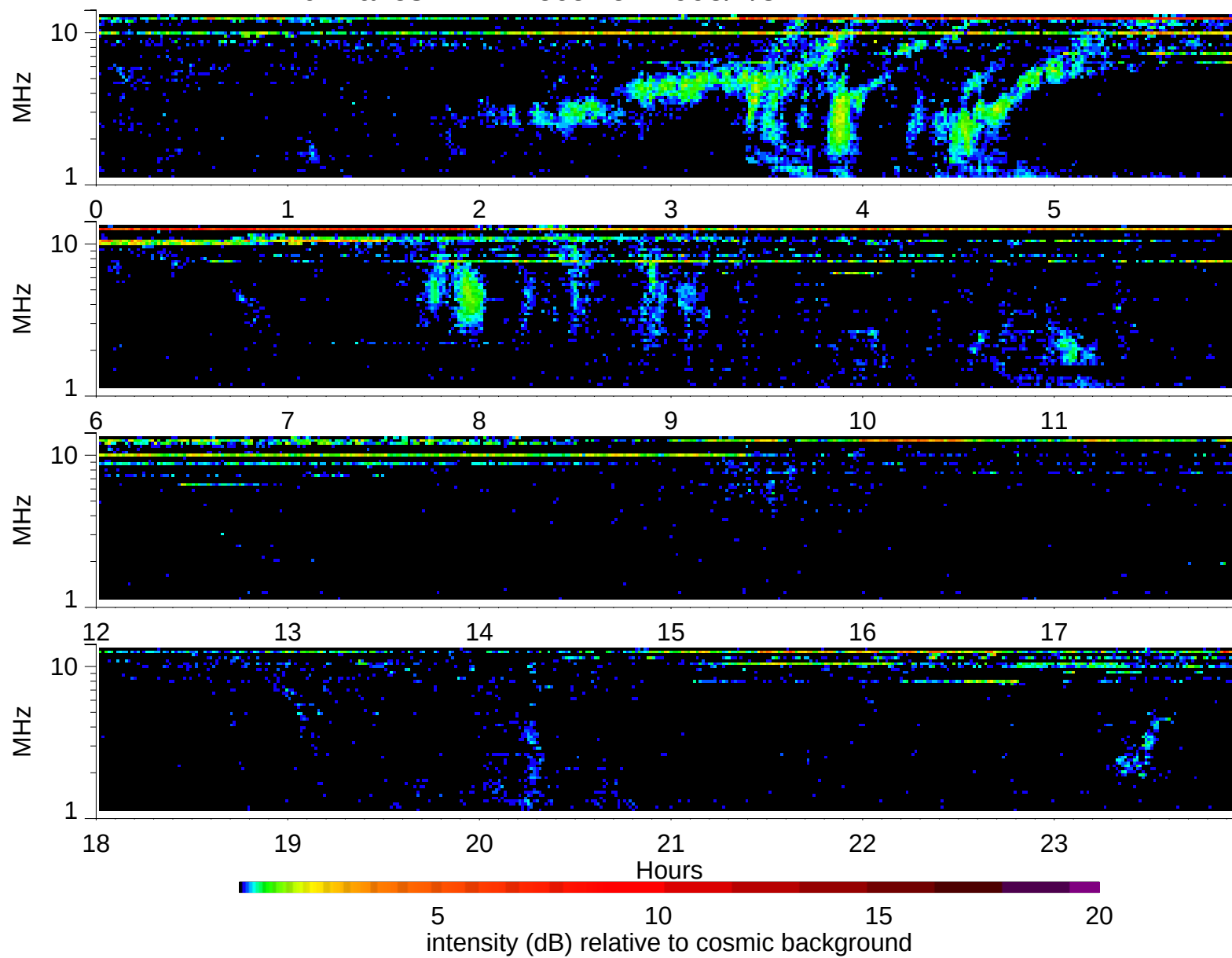
Wind Waves RAD2 receiver: 1995/7/8
