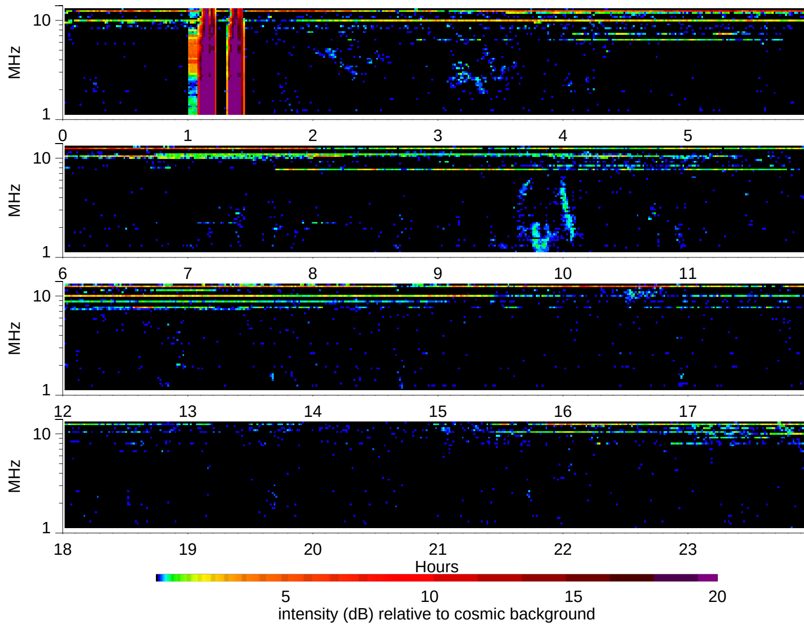
Wind Waves RAD2 receiver: 1995/7/13
