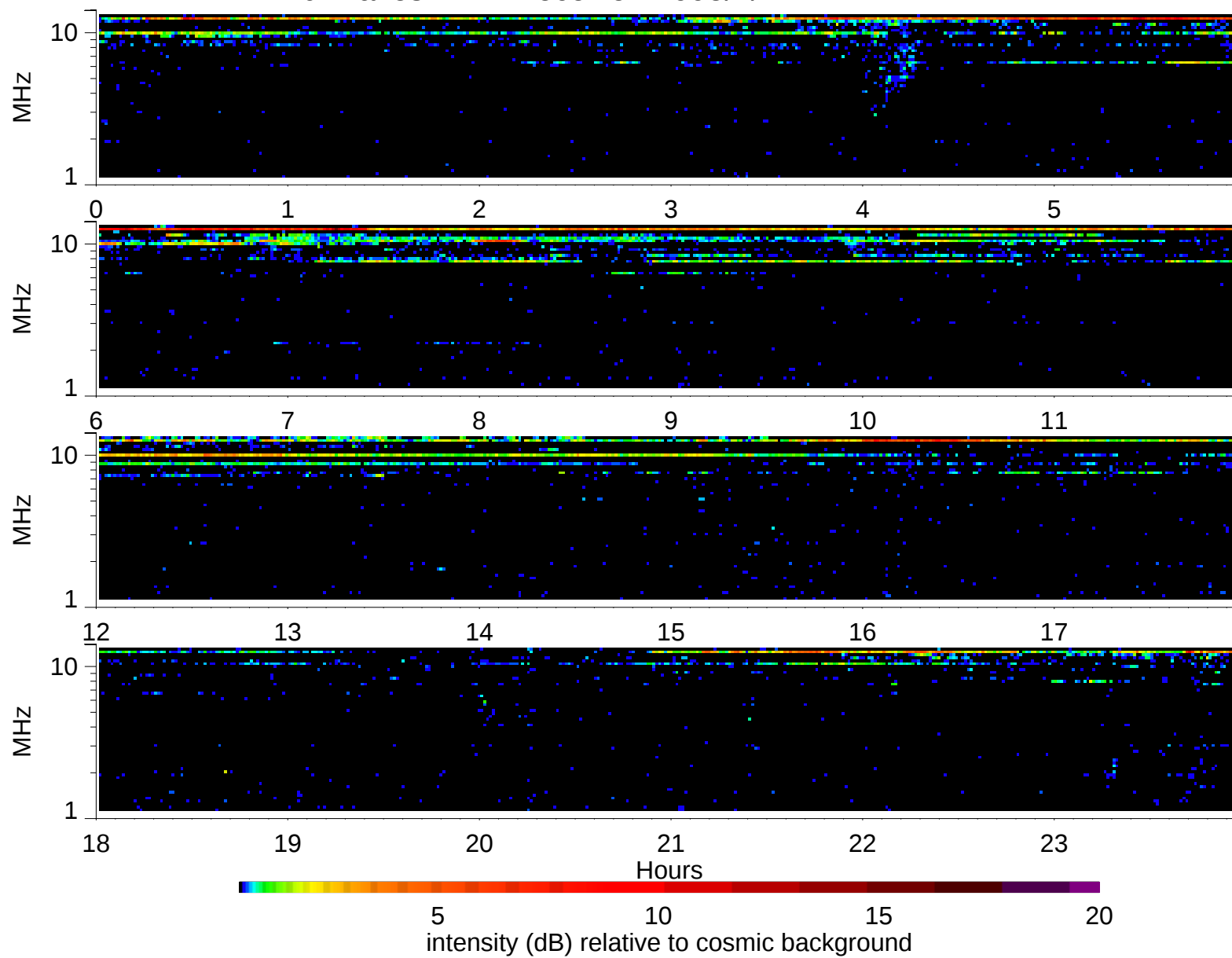
Wind Waves RAD2 receiver: 1995/7/14
