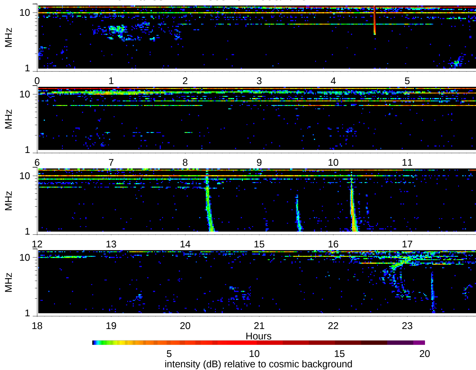
Wind Waves RAD2 receiver: 1995/7/16
