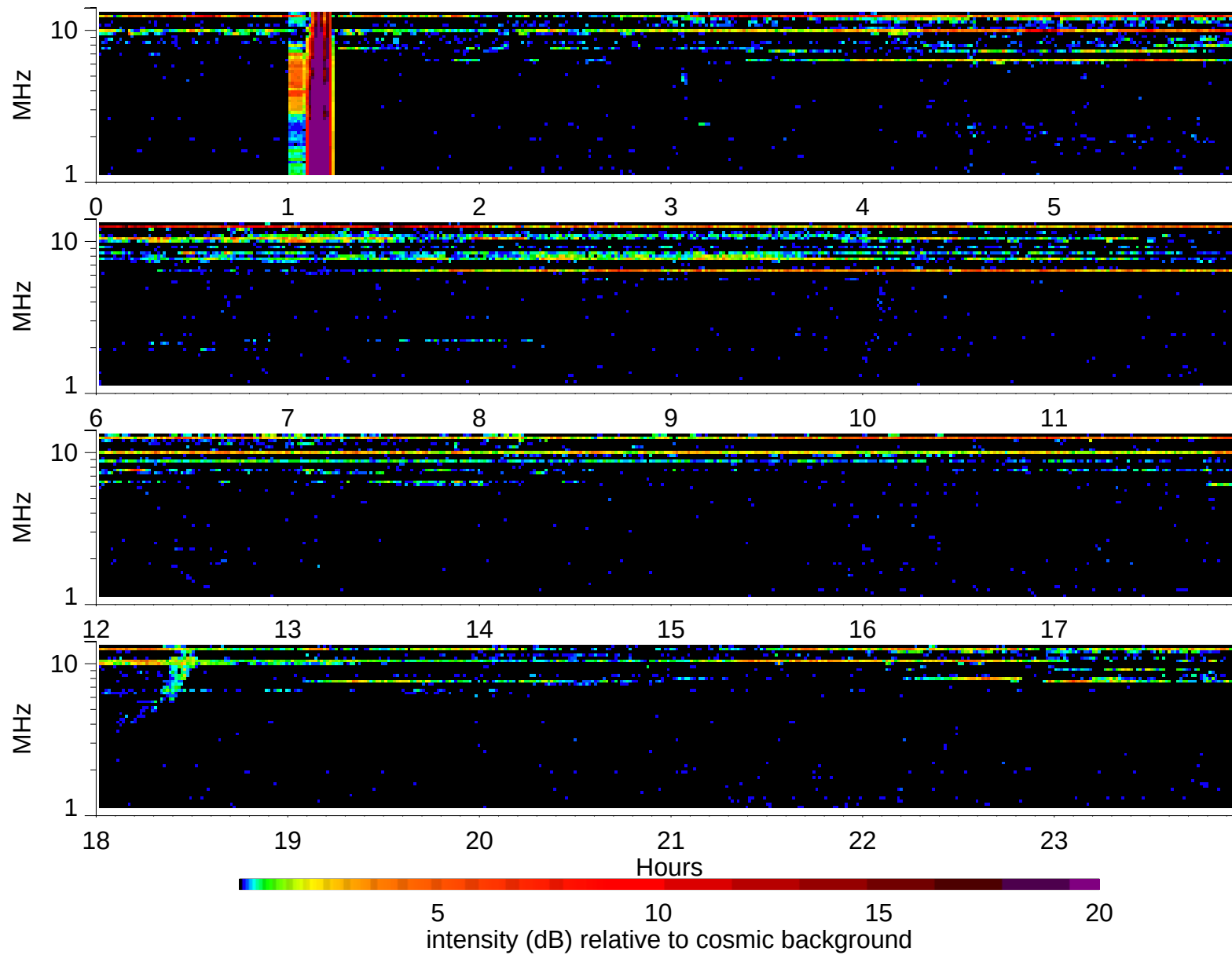
Wind Waves RAD2 receiver: 1995/7/17
