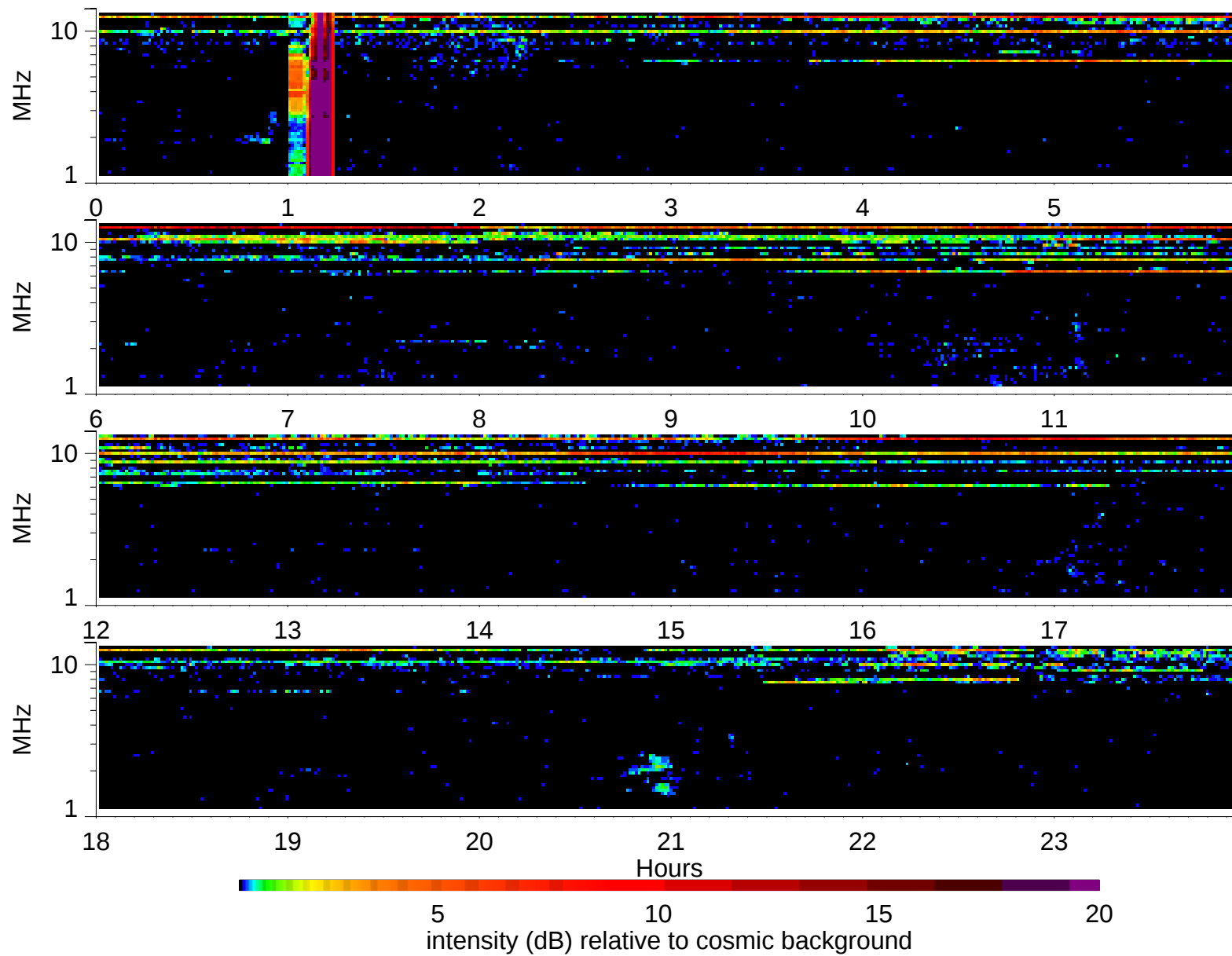
Wind Waves RAD2 receiver: 1995/7/23
