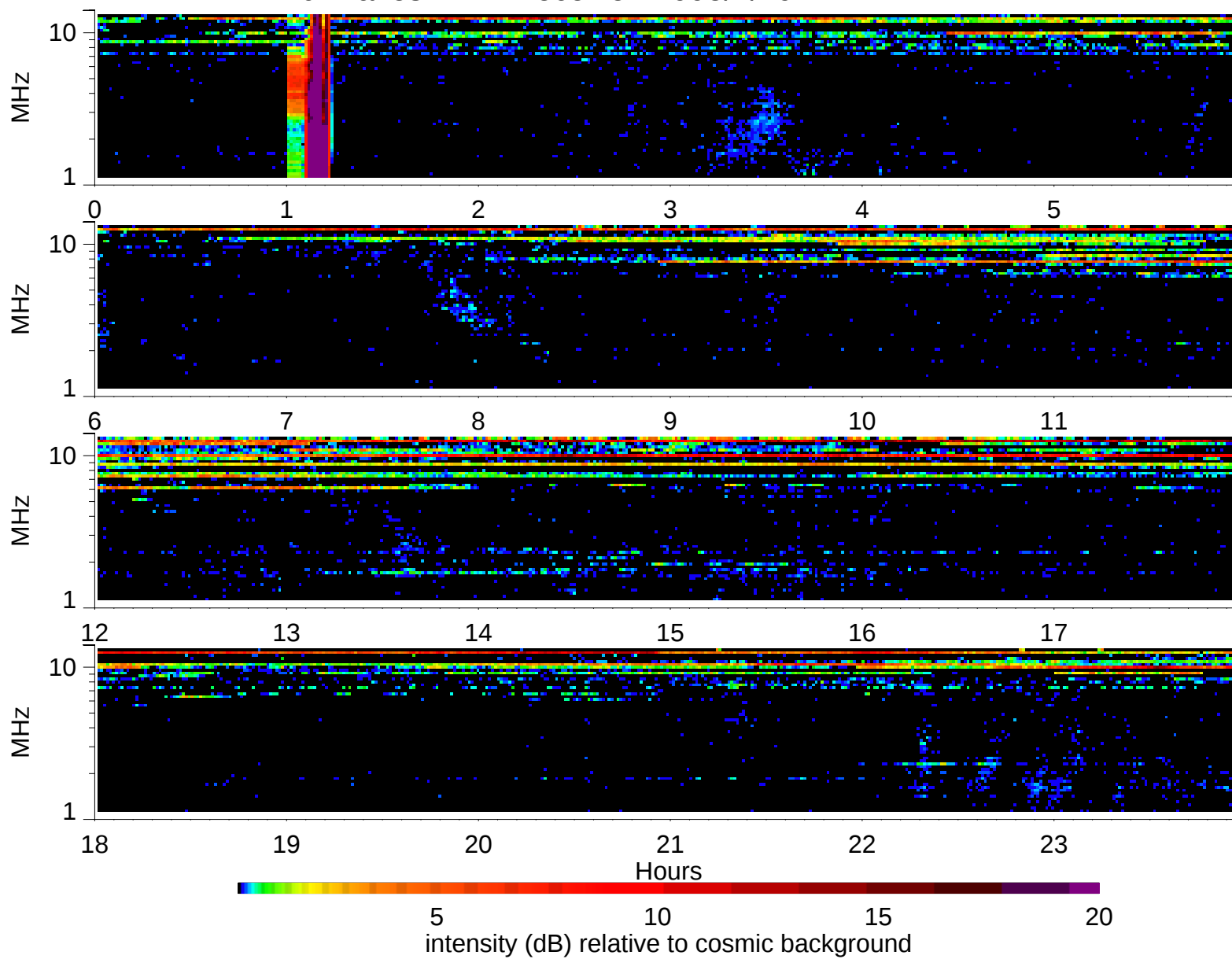
Wind Waves RAD2 receiver: 1995/7/29
