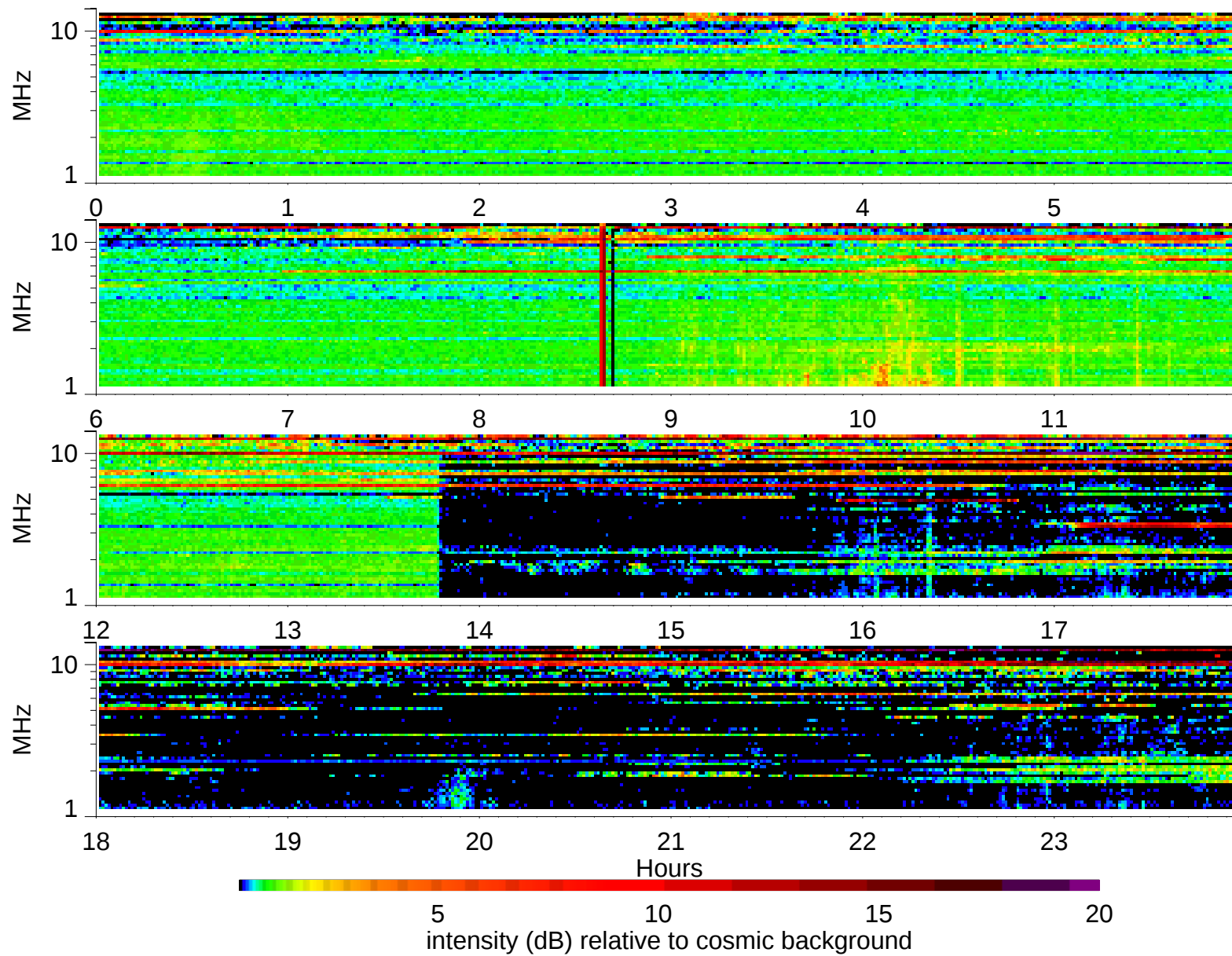
Wind Waves RAD2 receiver: 1995/8/1
