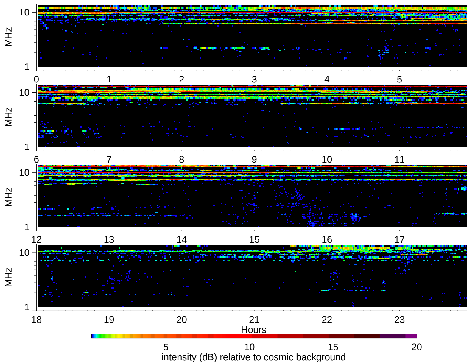
Wind Waves RAD2 receiver: 1995/8/7
