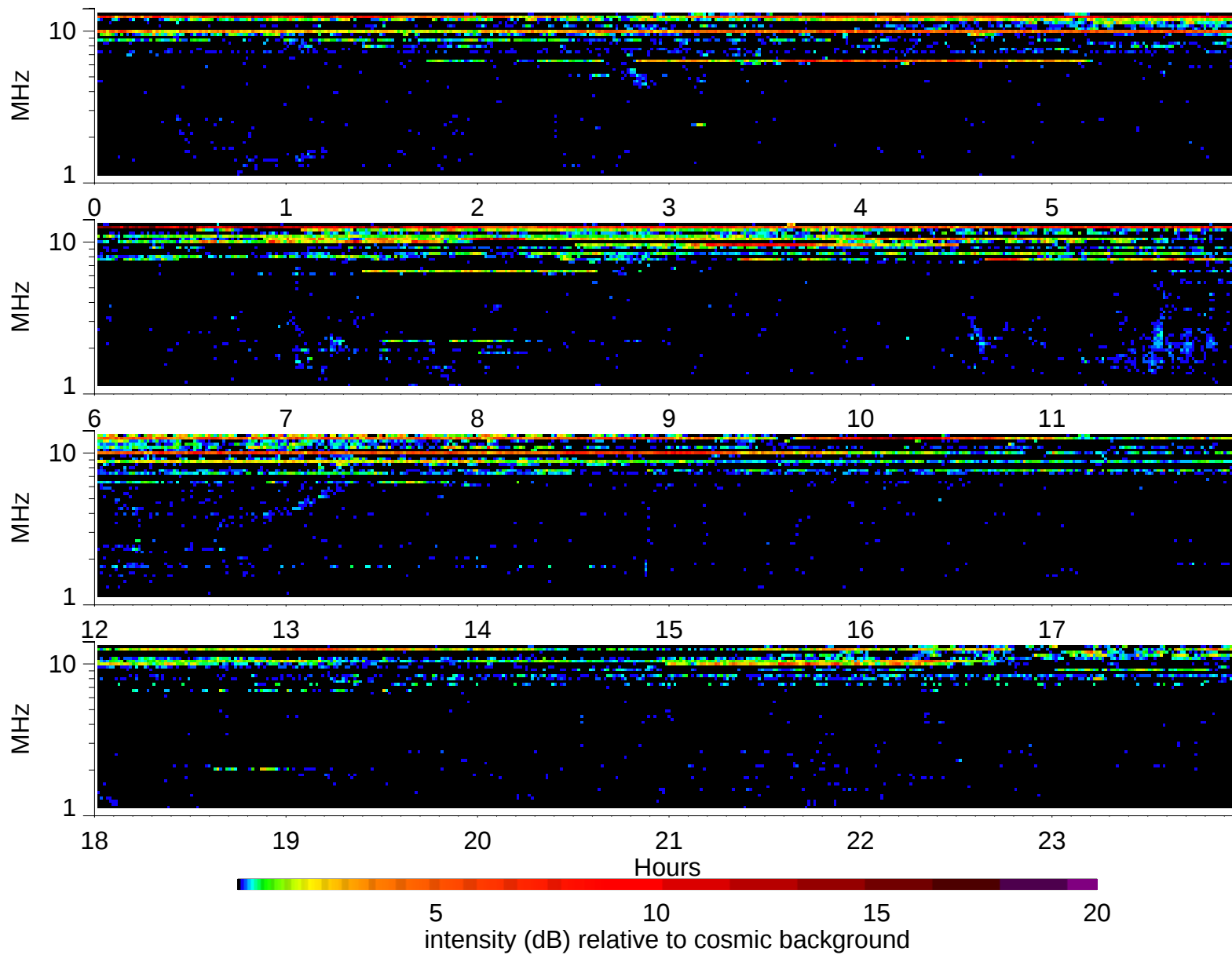
Wind Waves RAD2 receiver: 1995/8/11
