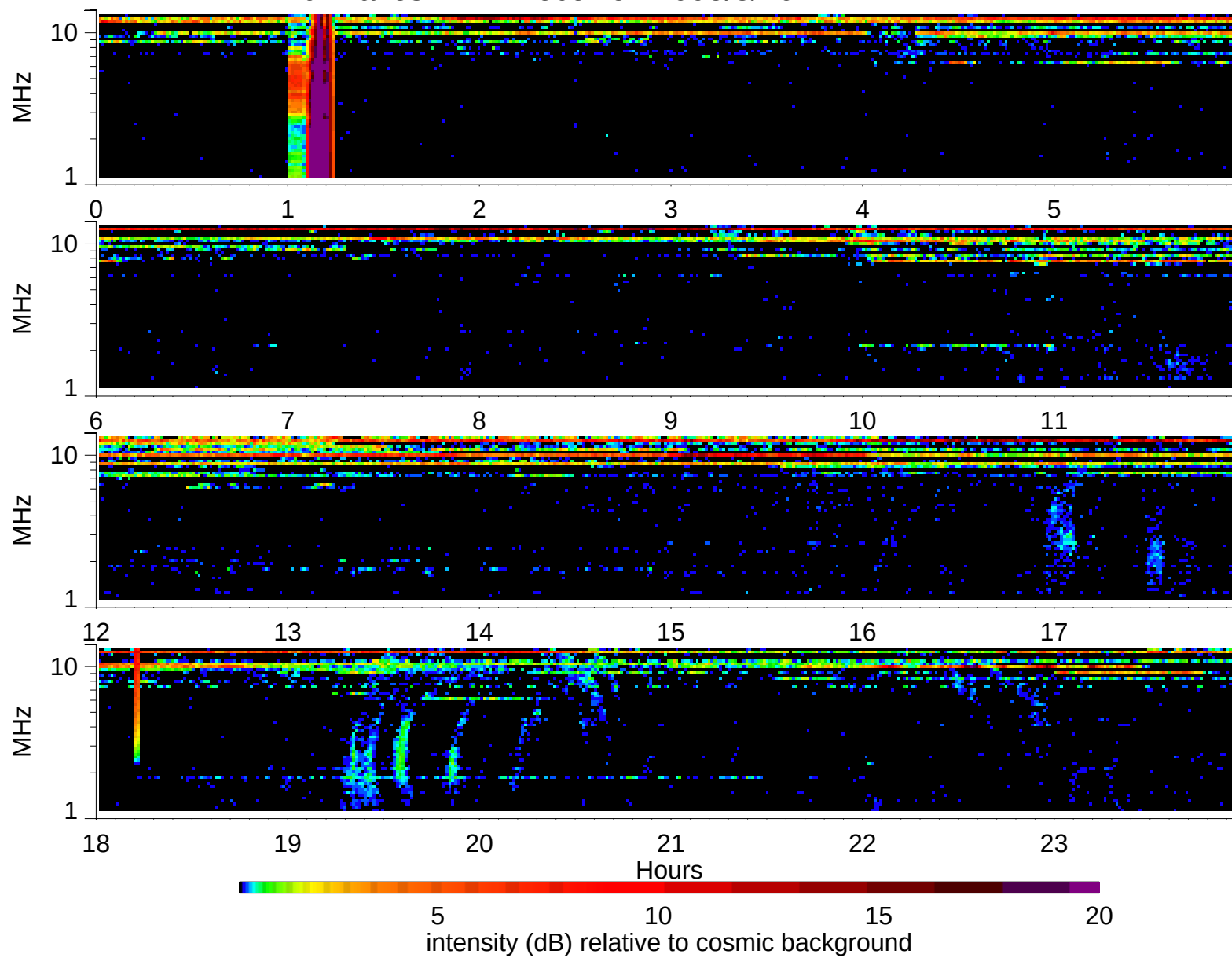
Wind Waves RAD2 receiver: 1995/8/16
