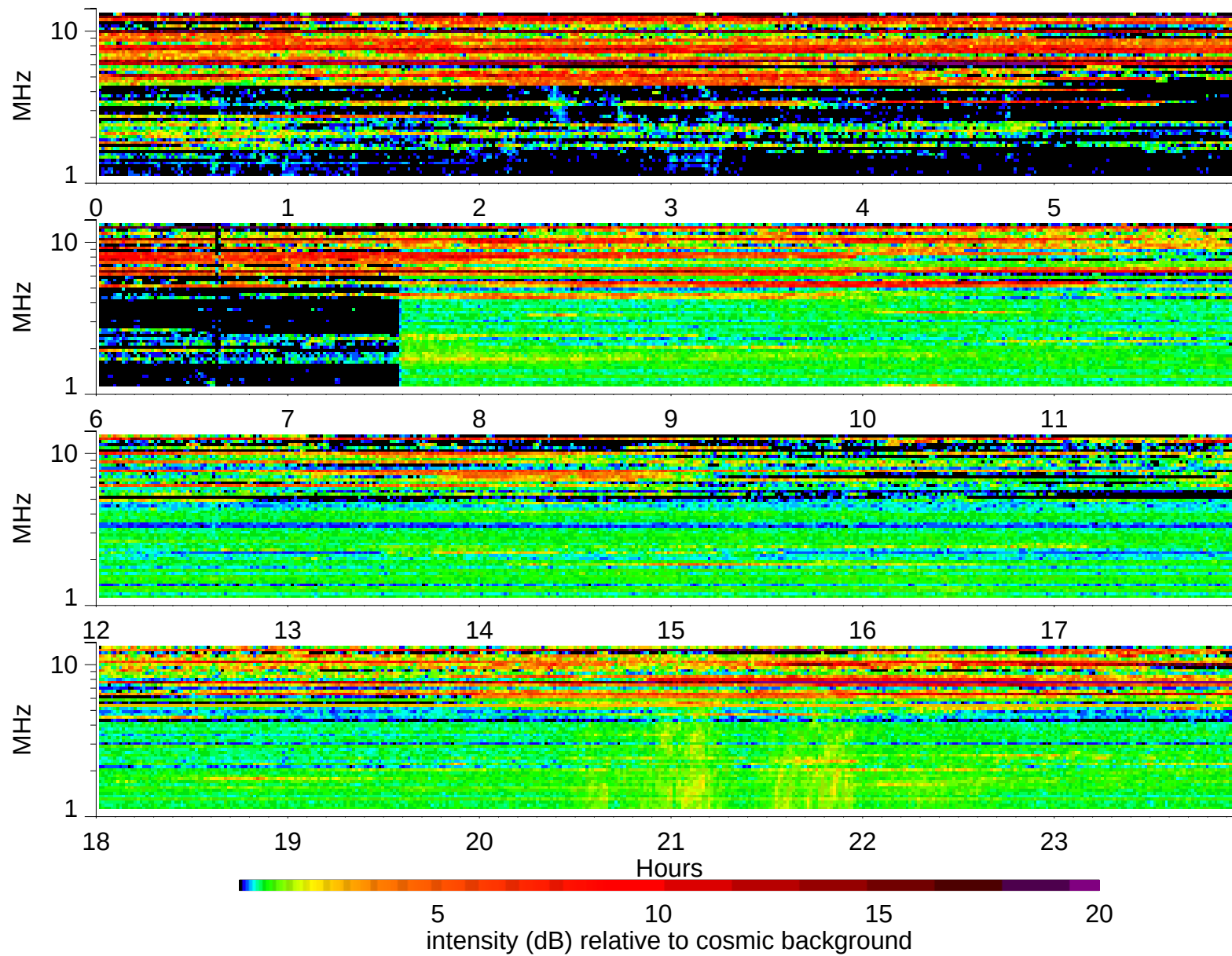
Wind Waves RAD2 receiver: 1995/8/21
