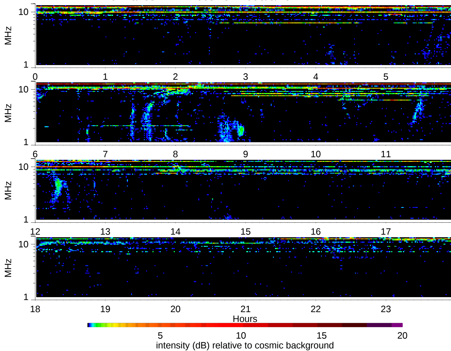
Wind Waves RAD2 receiver: 1995/8/29
