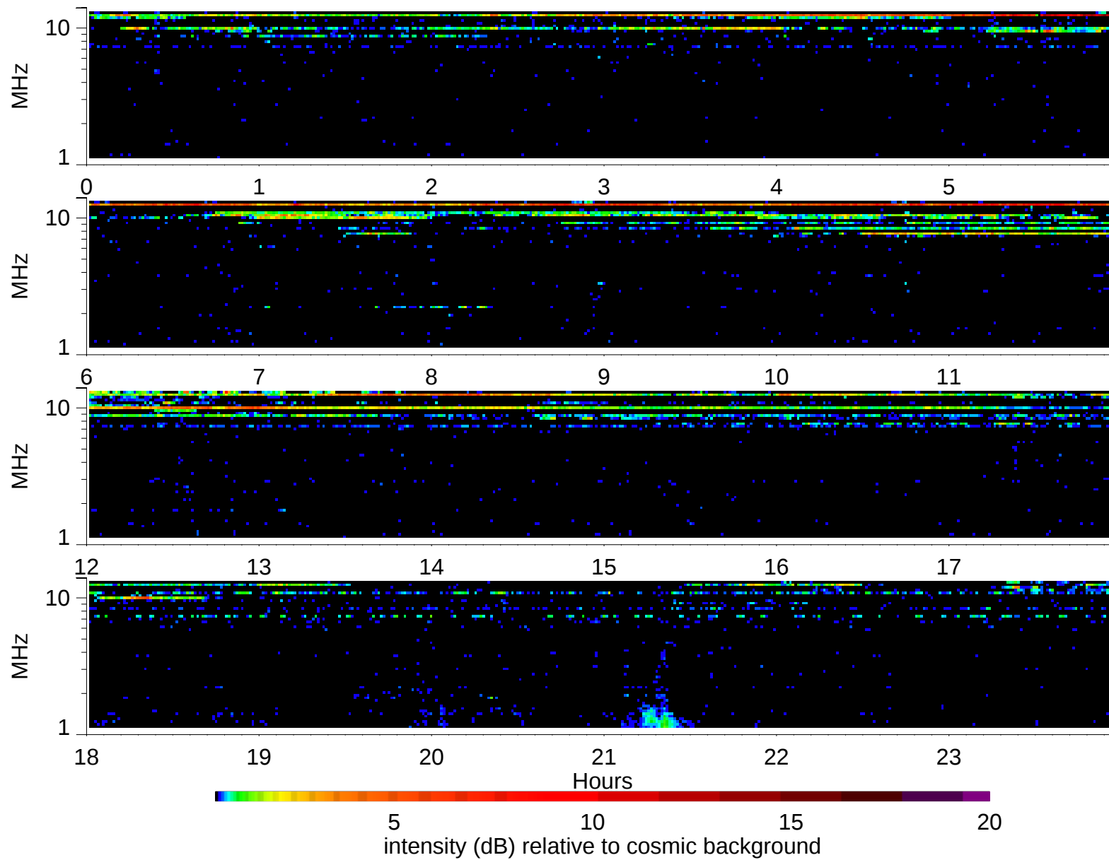
Wind Waves RAD2 receiver: 1995/9/2
