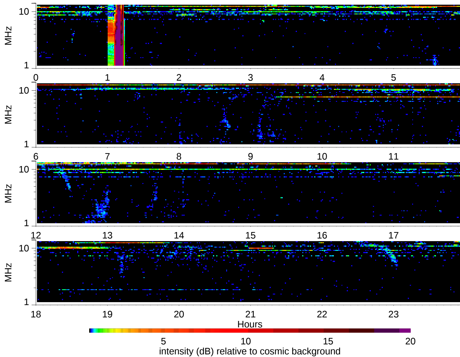
Wind Waves RAD2 receiver: 1995/9/9
