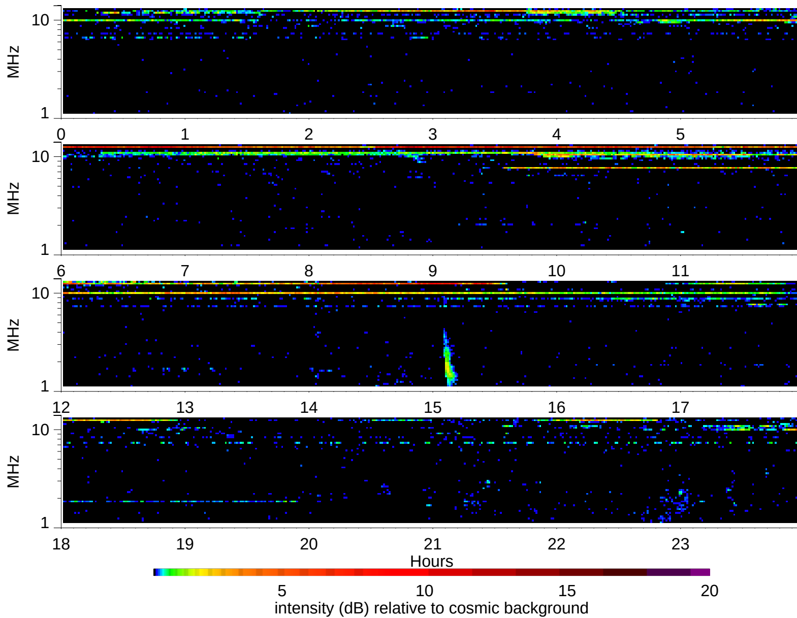
Wind Waves RAD2 receiver: 1995/9/10
