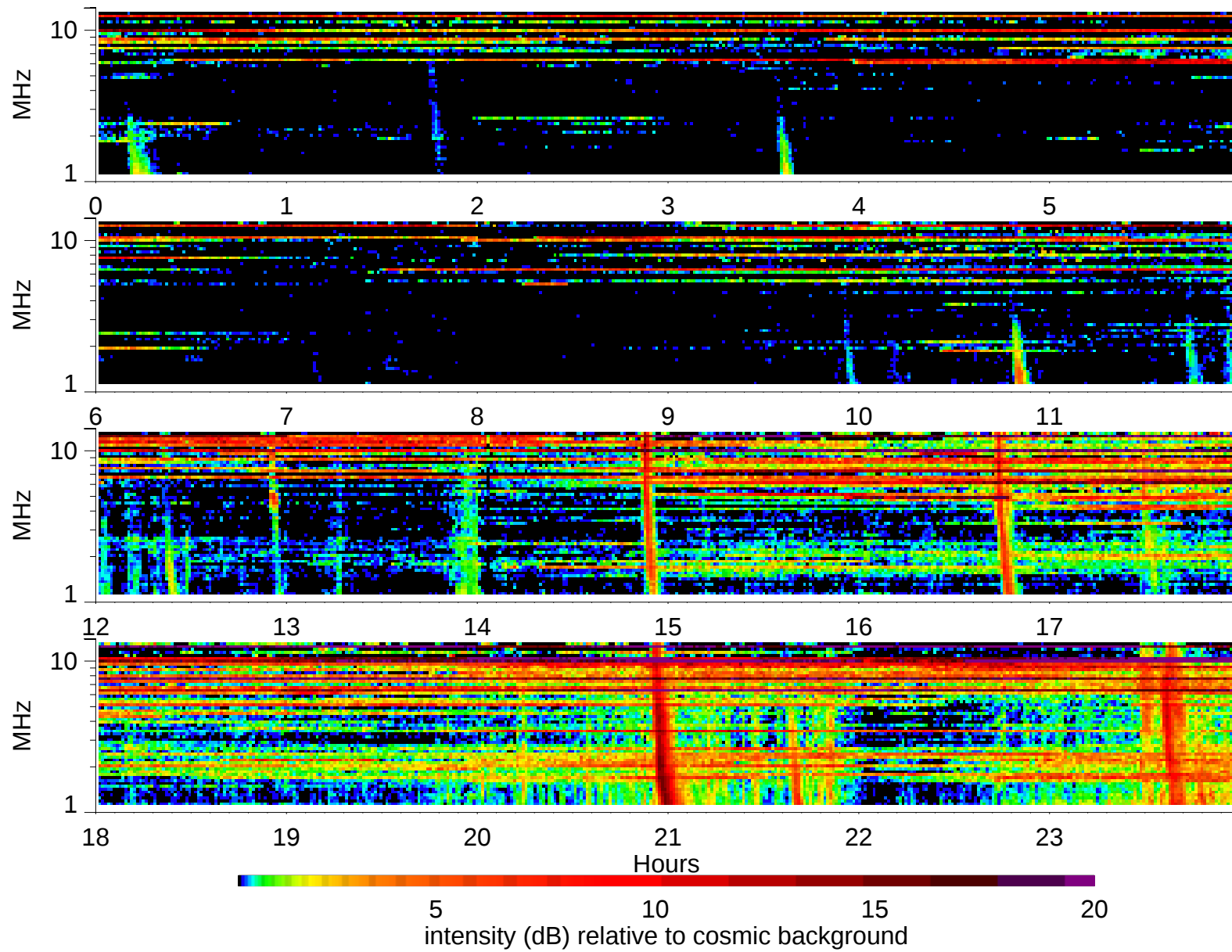
Wind Waves RAD2 receiver: 1995/9/16
