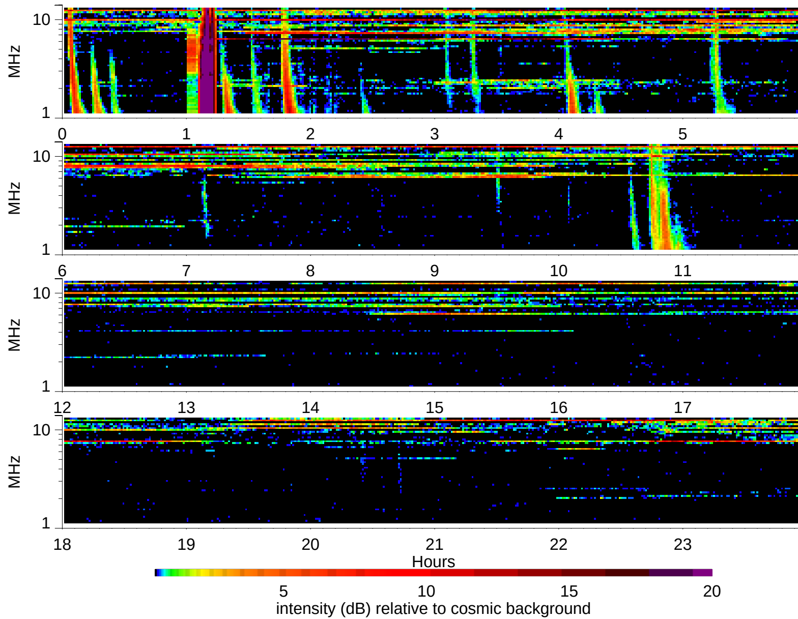
Wind Waves RAD2 receiver: 1995/9/23
