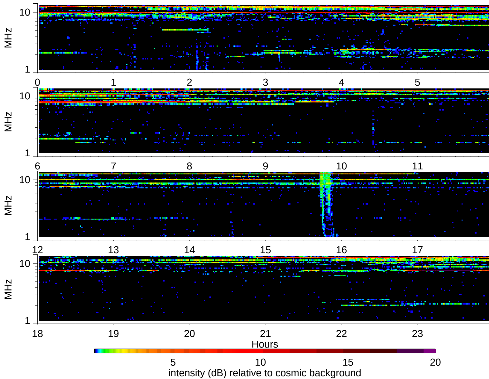
Wind Waves RAD2 receiver: 1995/9/24
