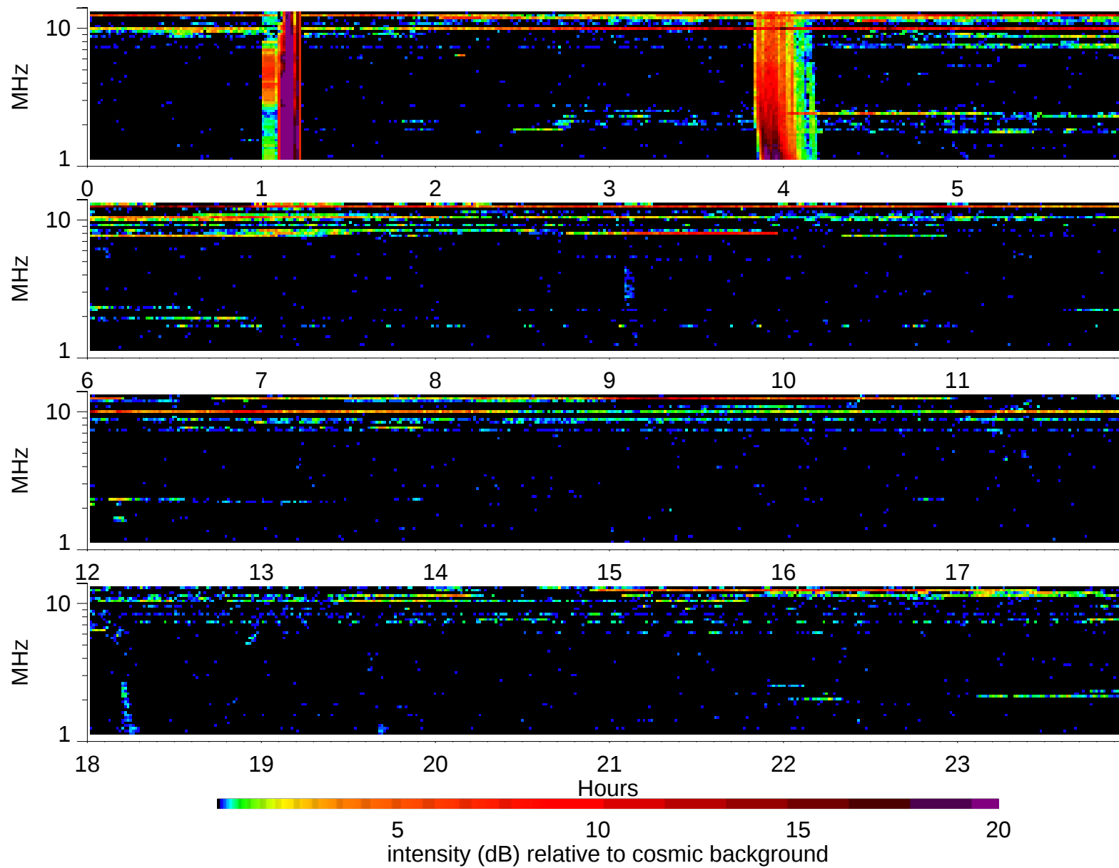
Wind Waves RAD2 receiver: 1995/9/25
