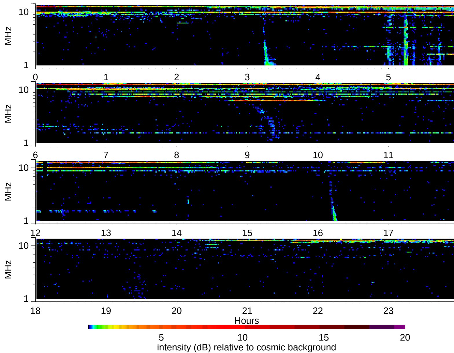
Wind Waves RAD2 receiver: 1995/9/28
