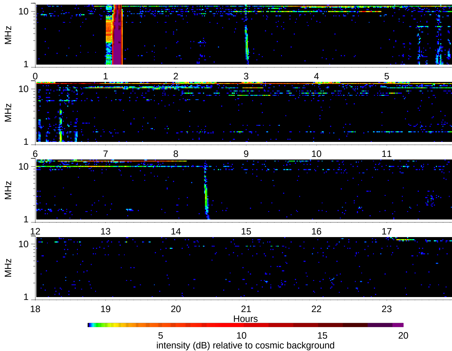
Wind Waves RAD2 receiver: 1995/10/5
