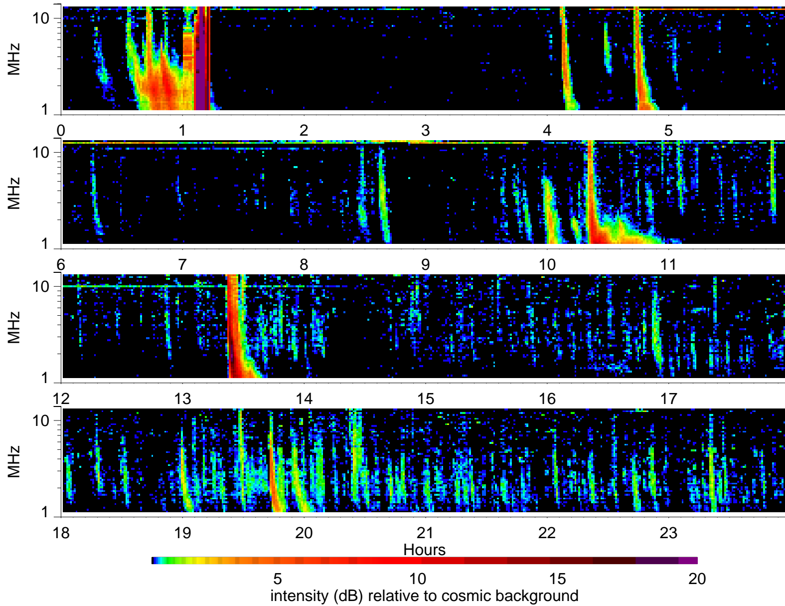
Wind Waves RAD2 receiver: 1995/10/15
