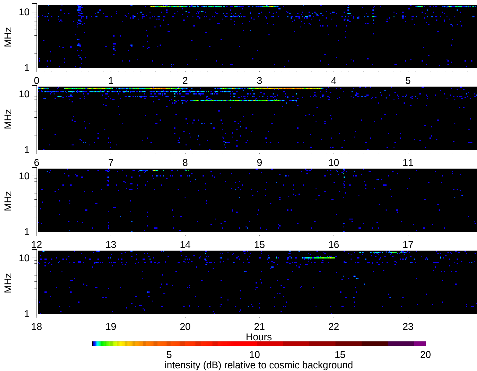
Wind Waves RAD2 receiver: 1995/10/22
