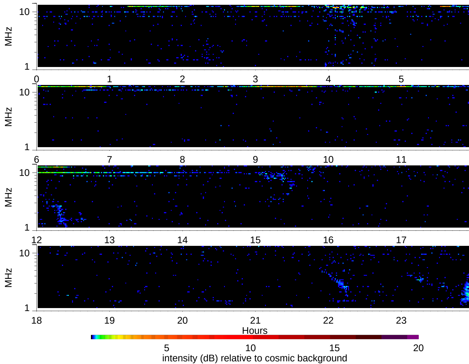
Wind Waves RAD2 receiver: 1995/10/26
