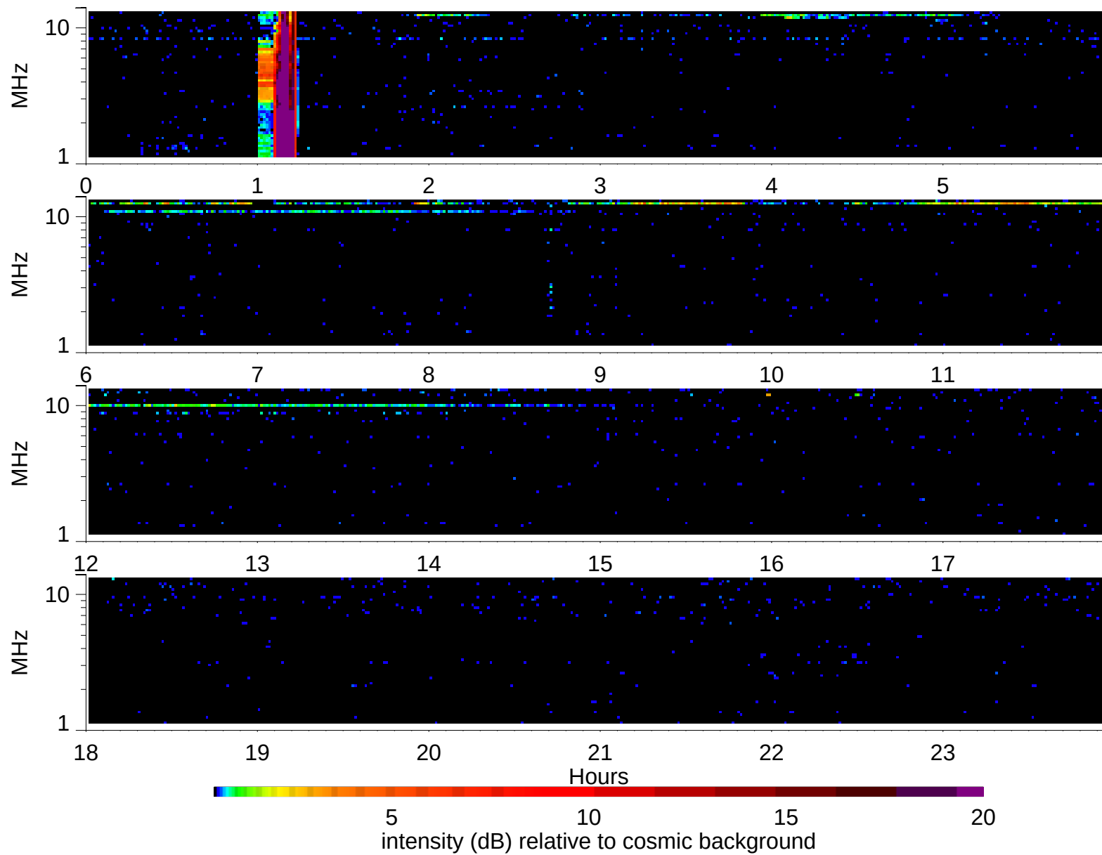
Wind Waves RAD2 receiver: 1995/10/29
