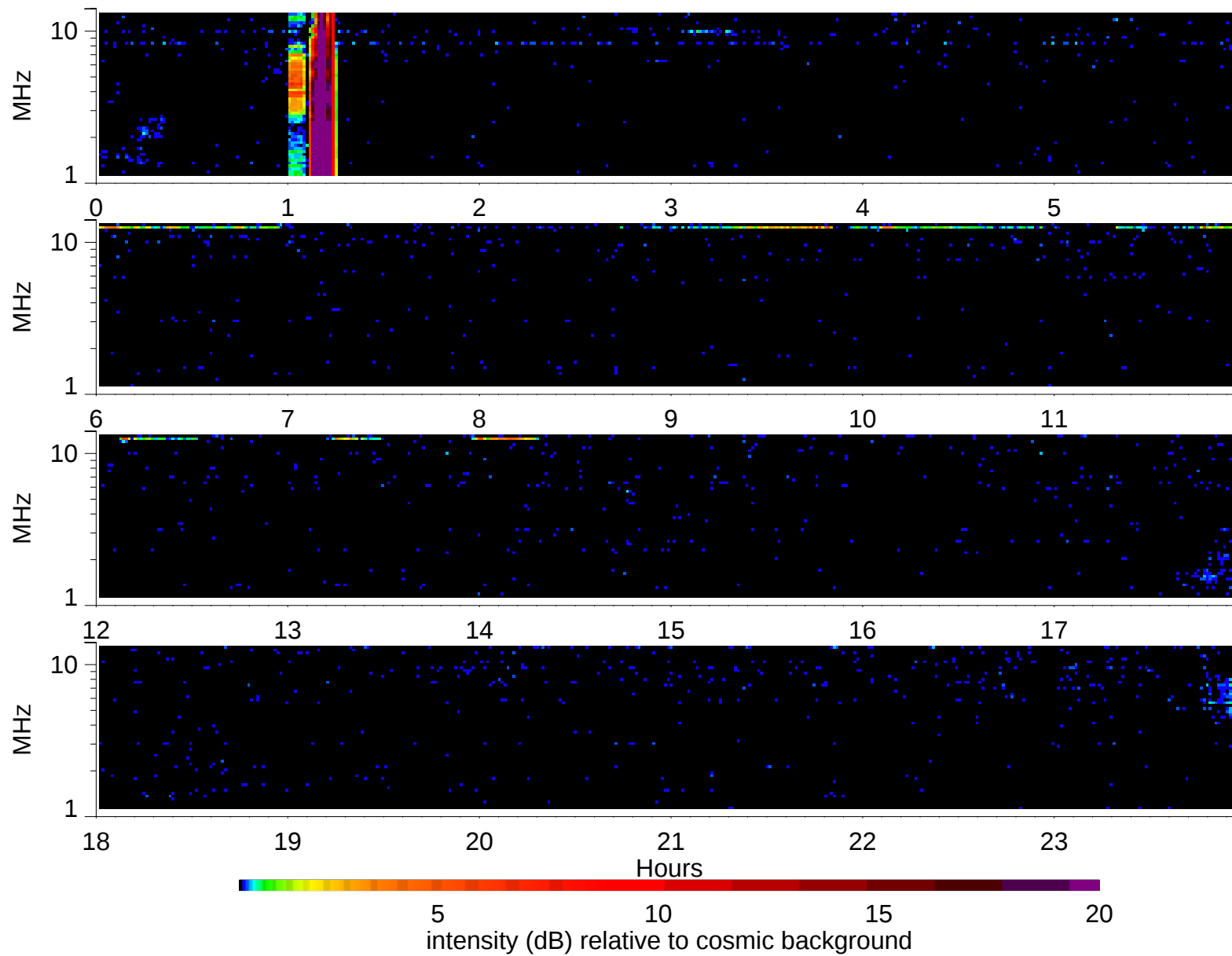
Wind Waves RAD2 receiver: 1995/11/8
