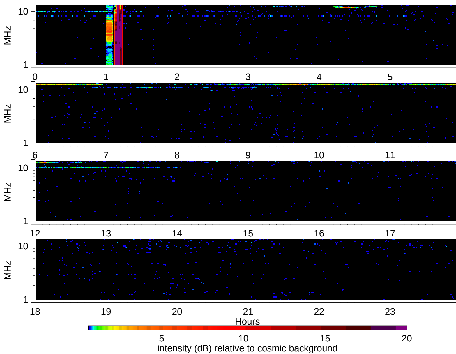
Wind Waves RAD2 receiver: 1995/11/10
