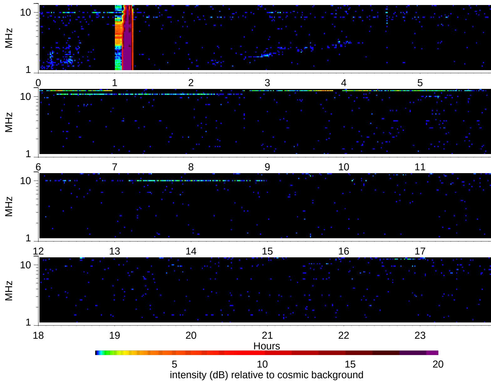
Wind Waves RAD2 receiver: 1995/11/12
