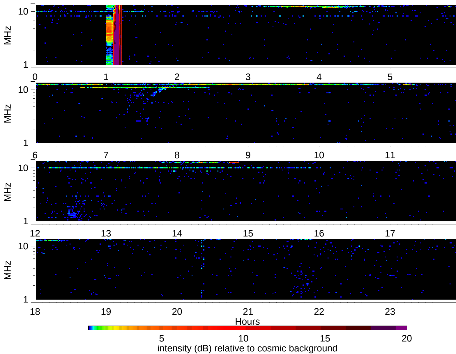
Wind Waves RAD2 receiver: 1995/11/14
