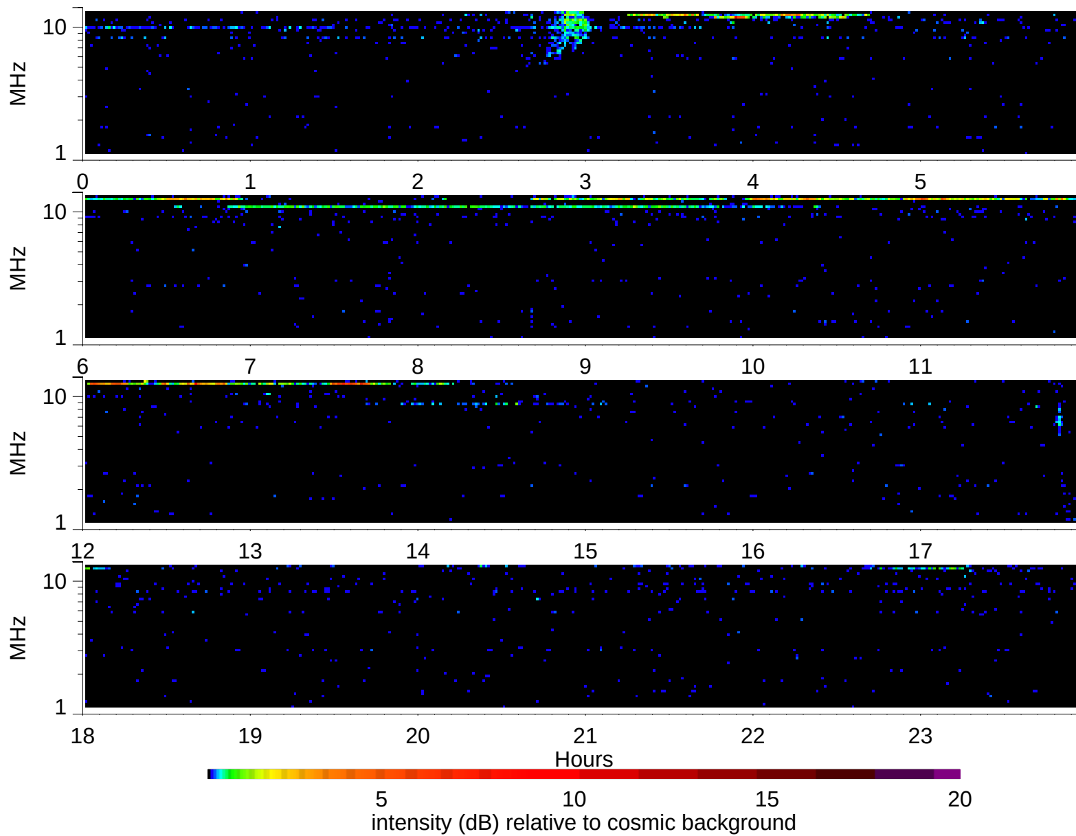
Wind Waves RAD2 receiver: 1995/11/15
