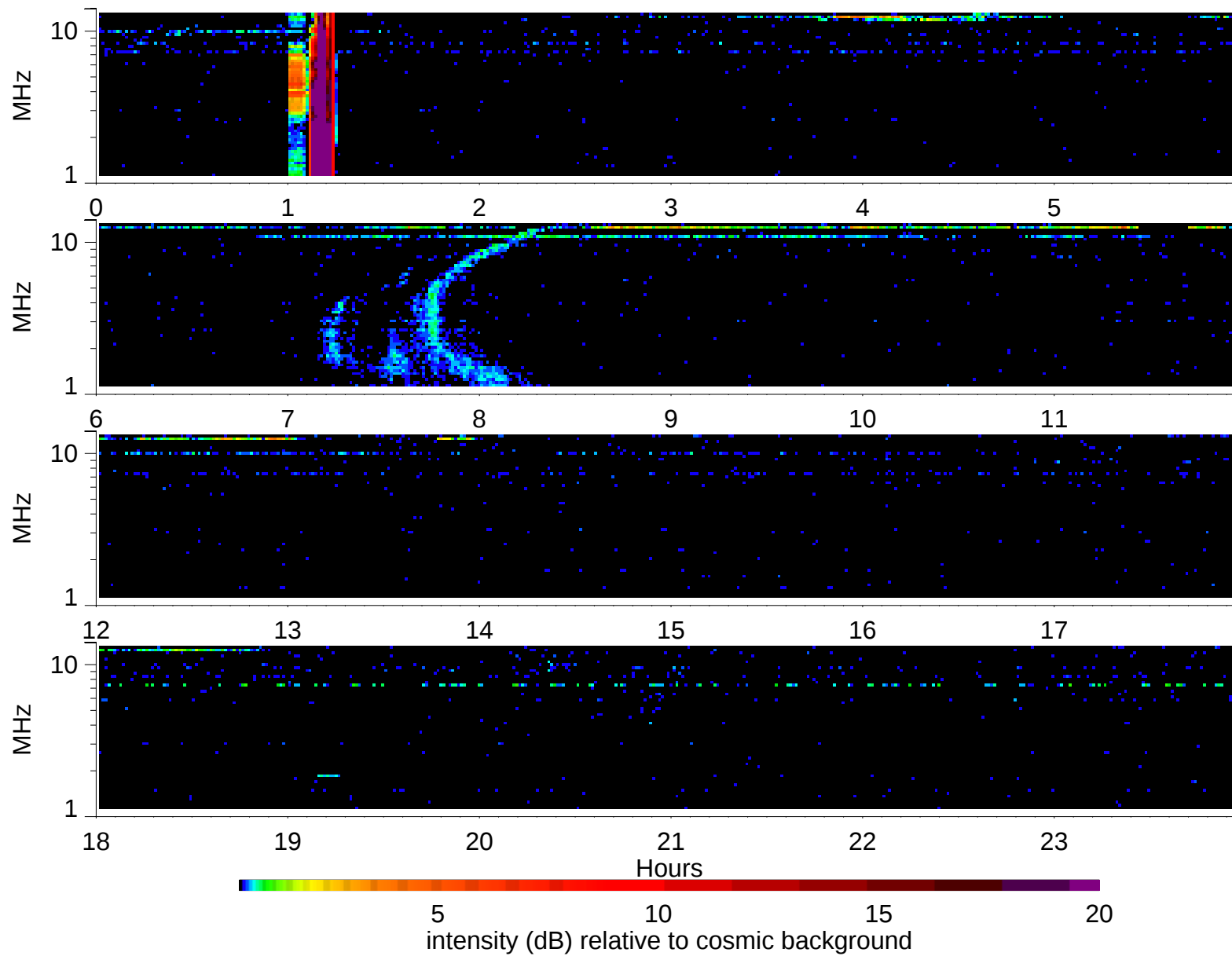
Wind Waves RAD2 receiver: 1995/11/16
