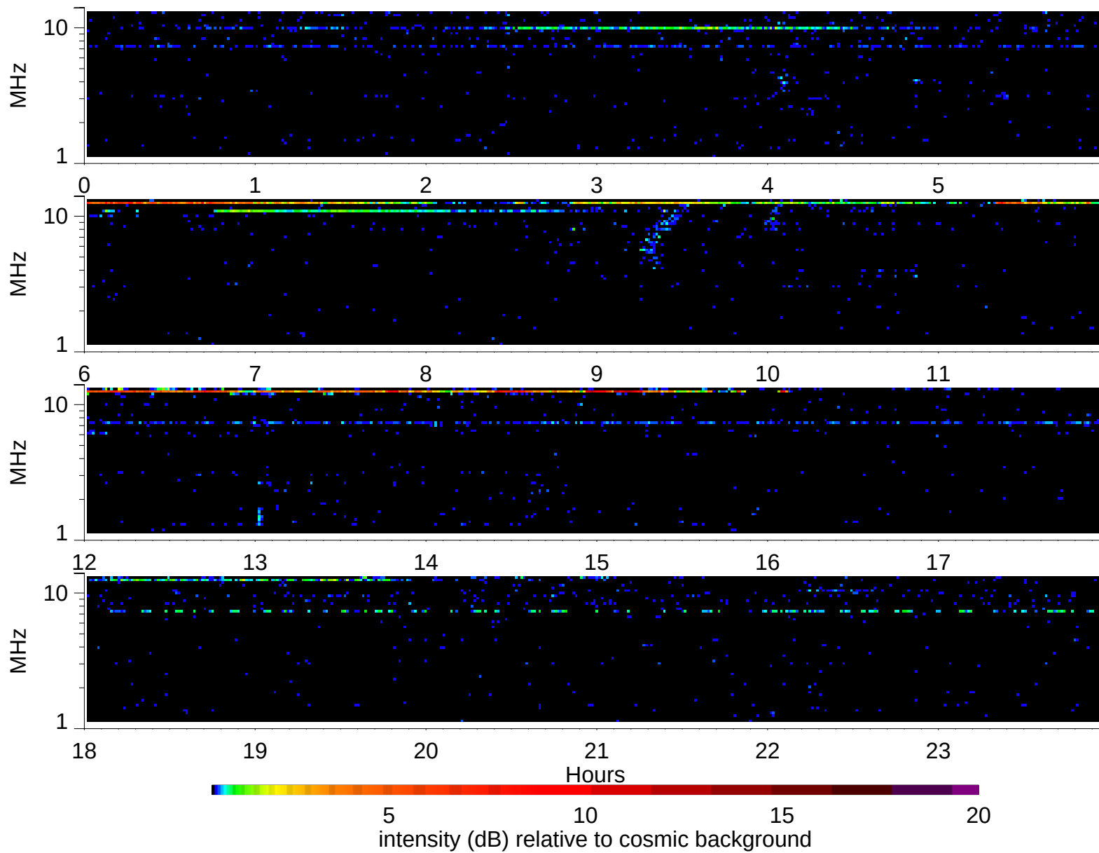
Wind Waves RAD2 receiver: 1995/11/21
