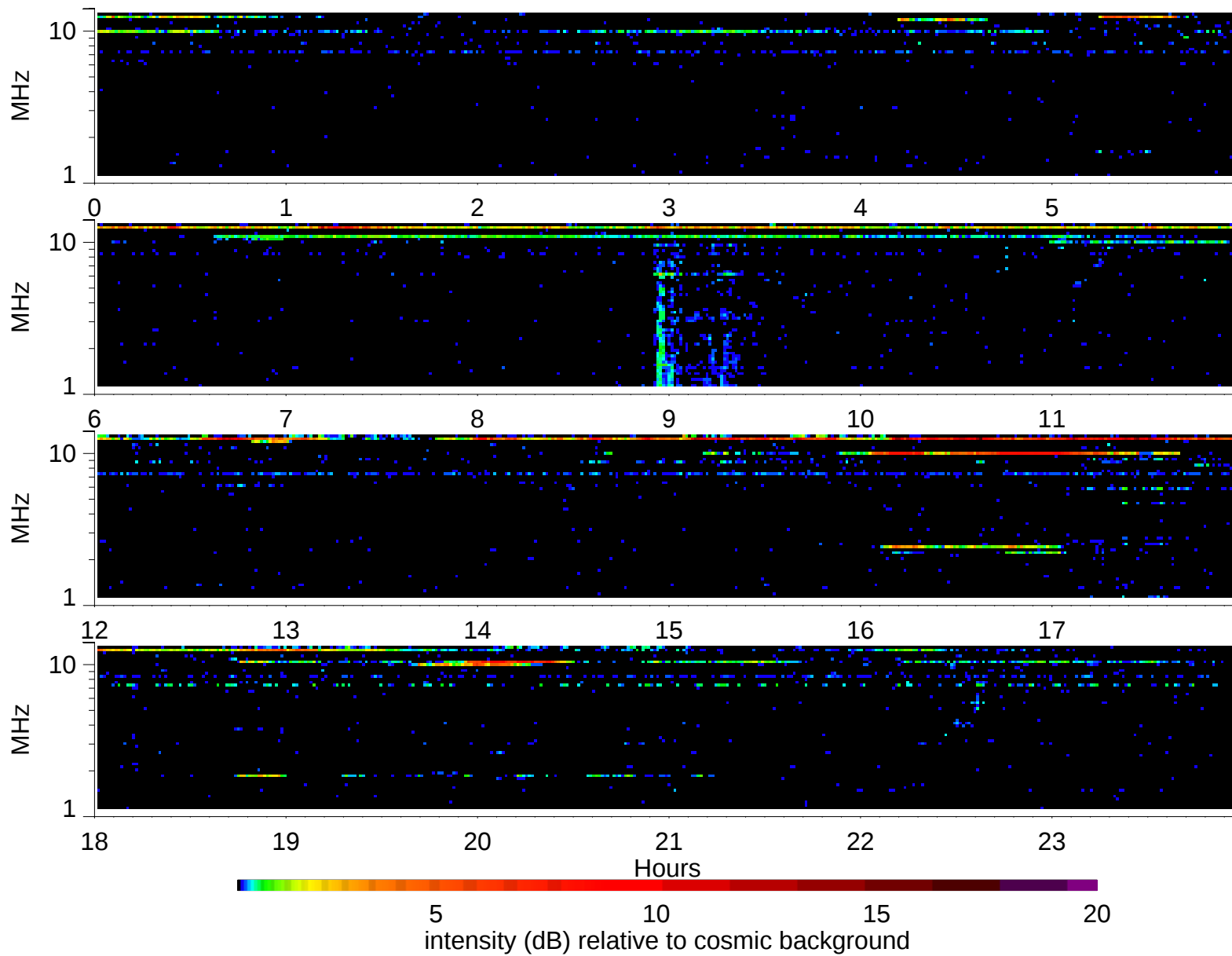
Wind Waves RAD2 receiver: 1995/11/23
