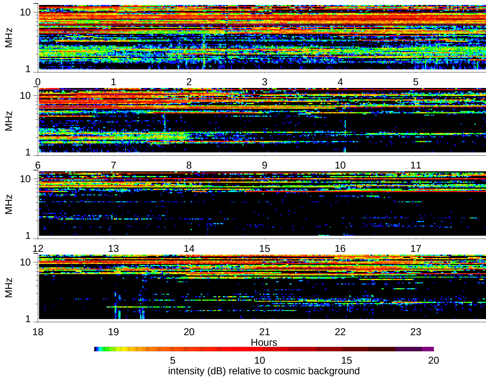
Wind Waves RAD2 receiver: 1995/11/30
