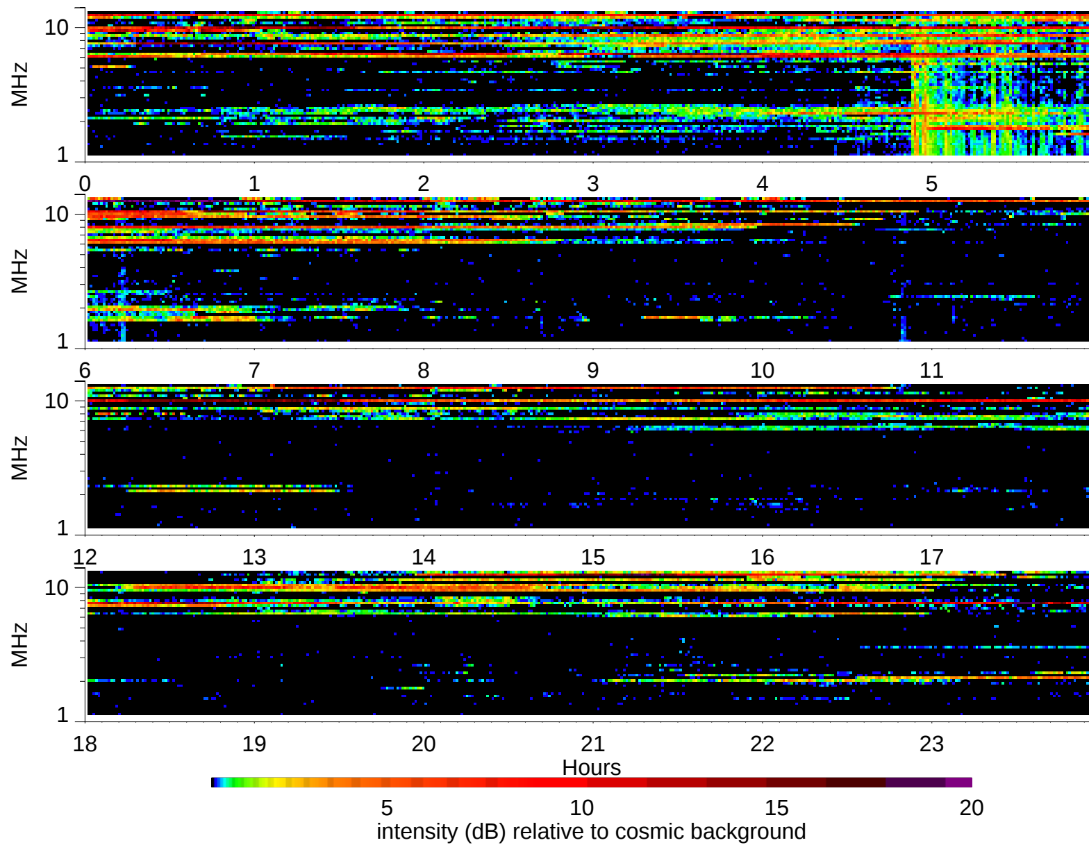
Wind Waves RAD2 receiver: 1995/12/1
