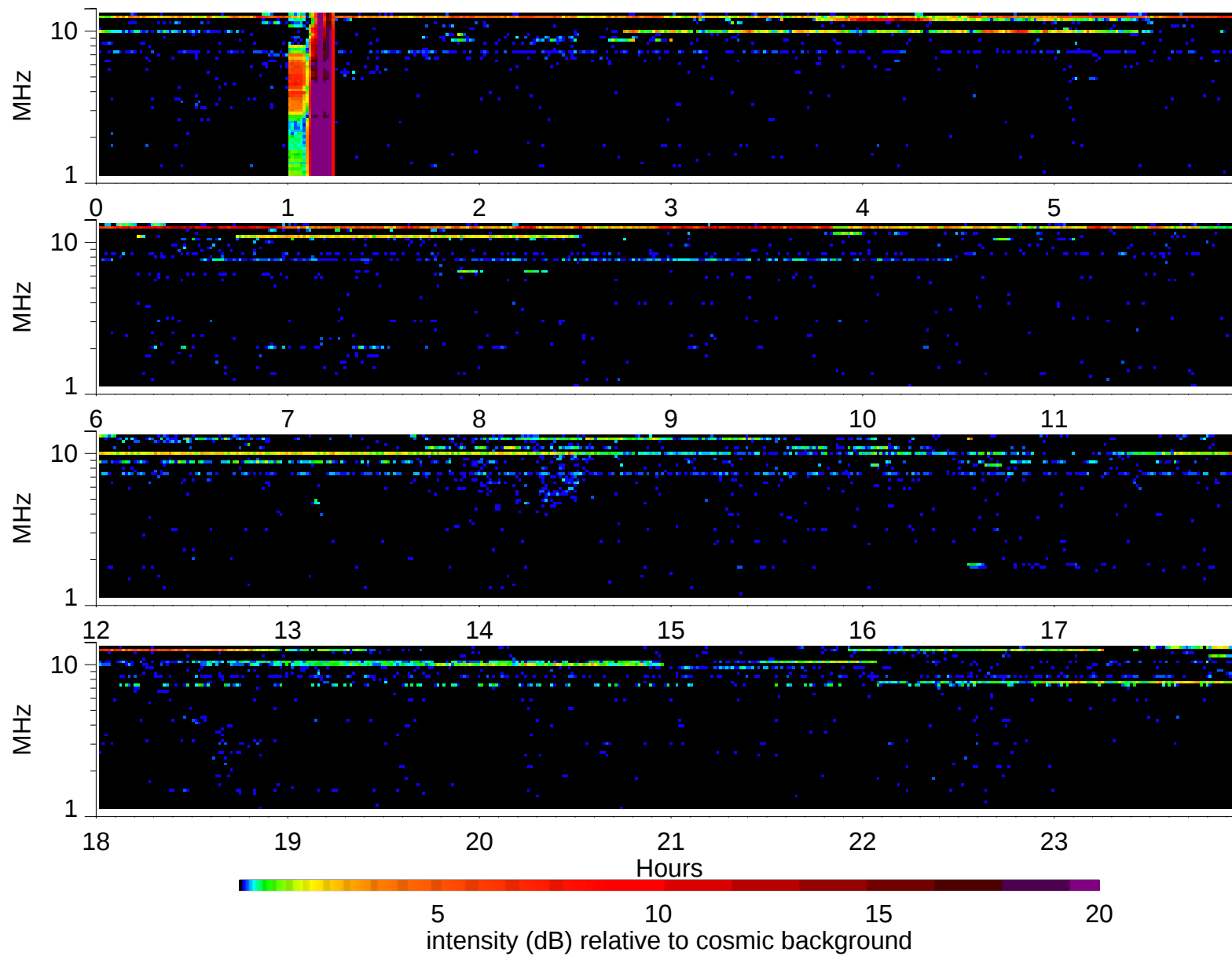
Wind Waves RAD2 receiver: 1995/12/4
