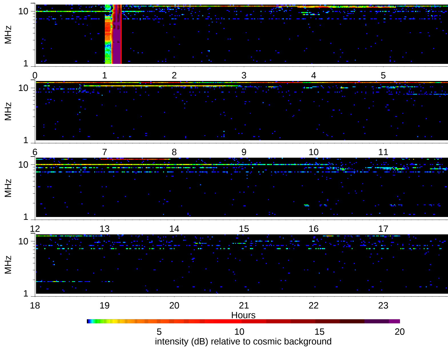
Wind Waves RAD2 receiver: 1995/12/8
