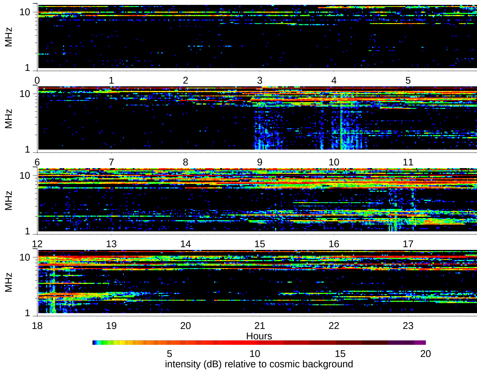
Wind Waves RAD2 receiver: 1995/12/19
